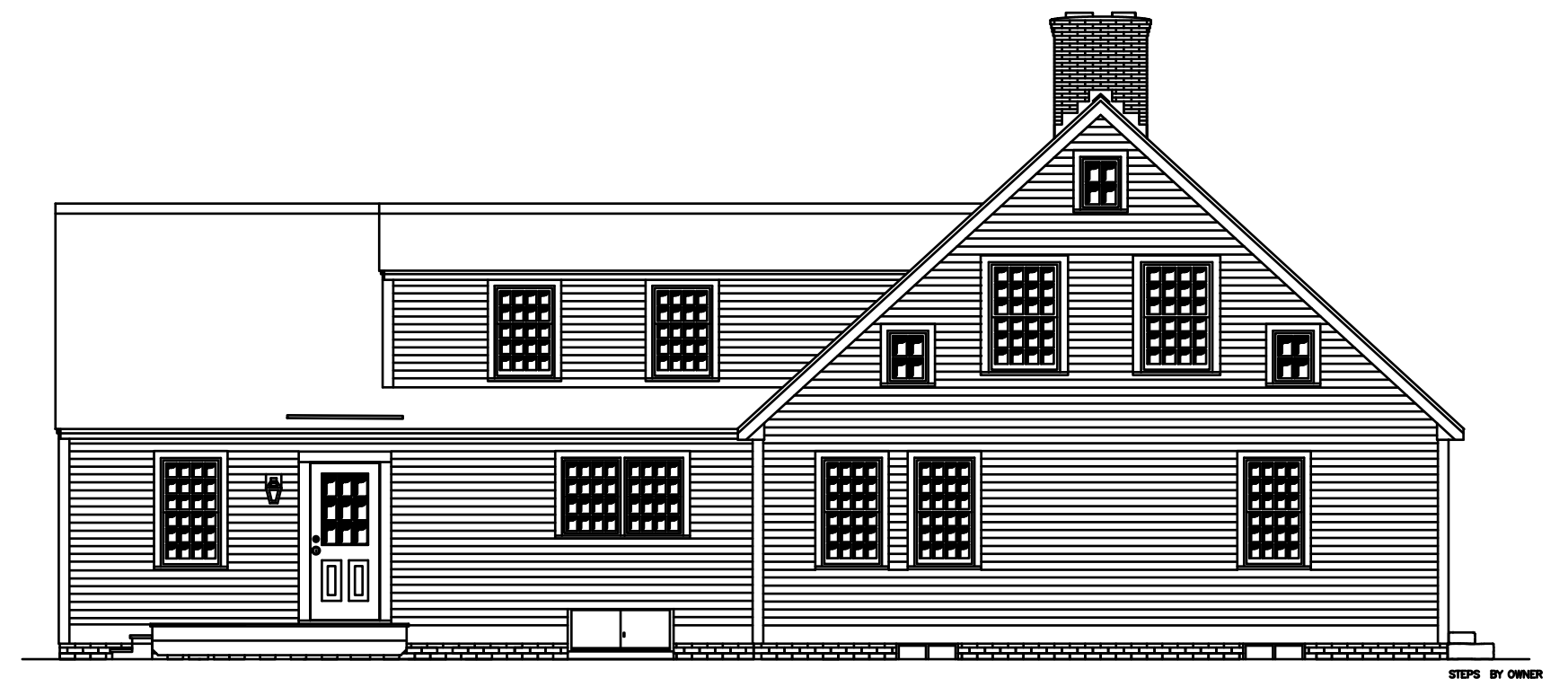
LEFT ELEVATION – NO SCALE
